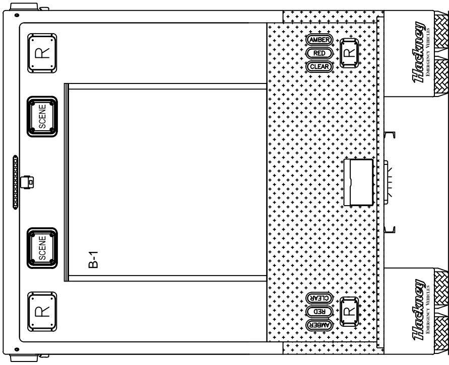
REAR VIEW
